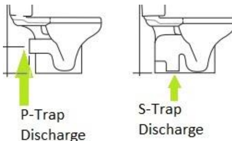
Figure 6.1 – Types of WC Discharge
