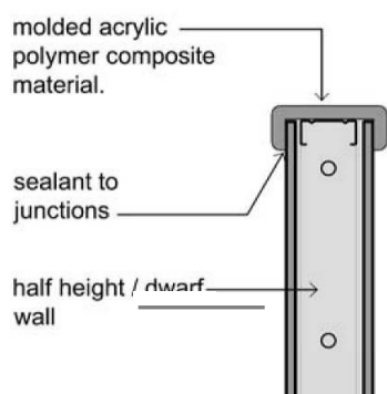
Figure 24: Recommended detail - low height wall capping
