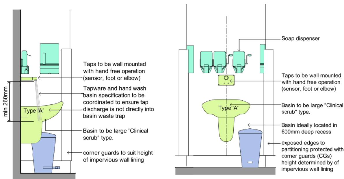
Figure 5: Type A Handwash basin
