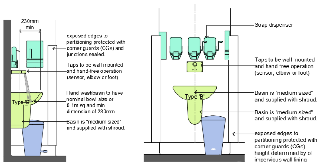
Figure 6: Type B Handwash basin
