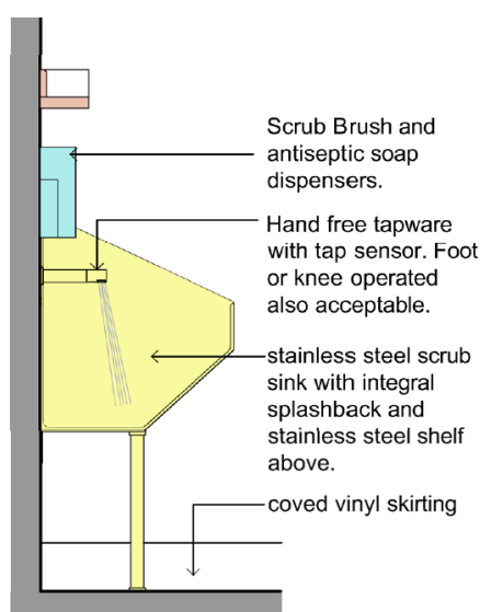
Figure 8: Typical scrub sink
