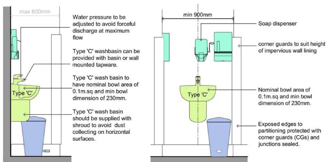
Figure 7: Type C Handwash basin
