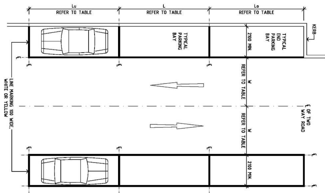
Figure 16: Parallel parking on both sides of a two way aisle
