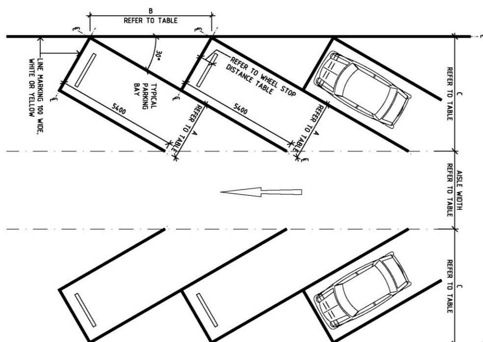
Figure 10: Typical Carparking Bays at 30°
